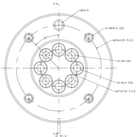
Flange drawing
