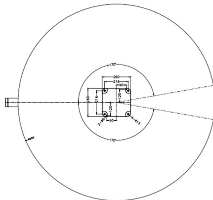
Base installation drawing
